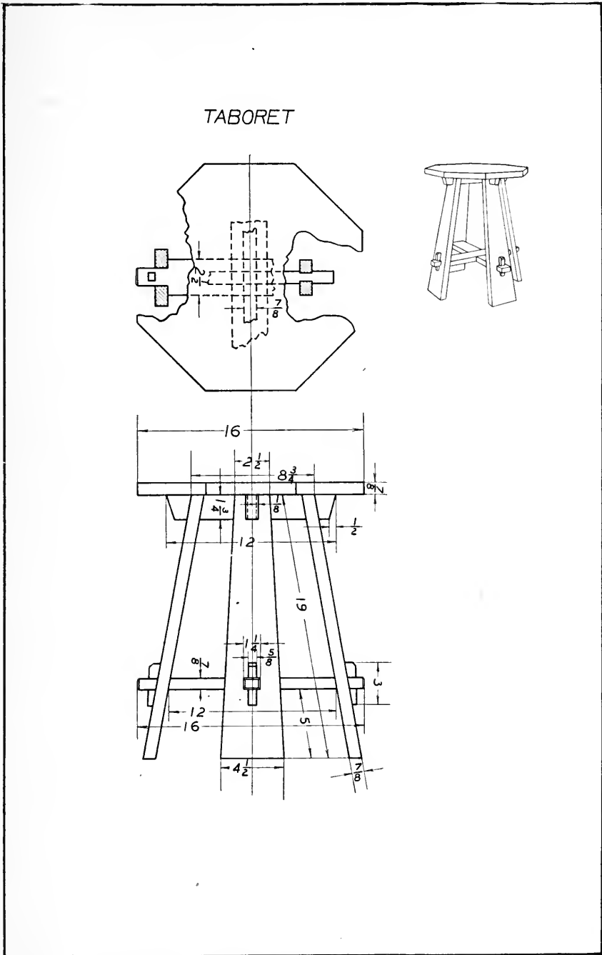
FIG. 384. POSSIBILITIES OF KEYED TENON.
